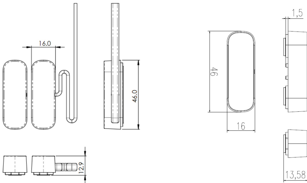
Reed Switch (46mm x 16mm x 12.9mm)
